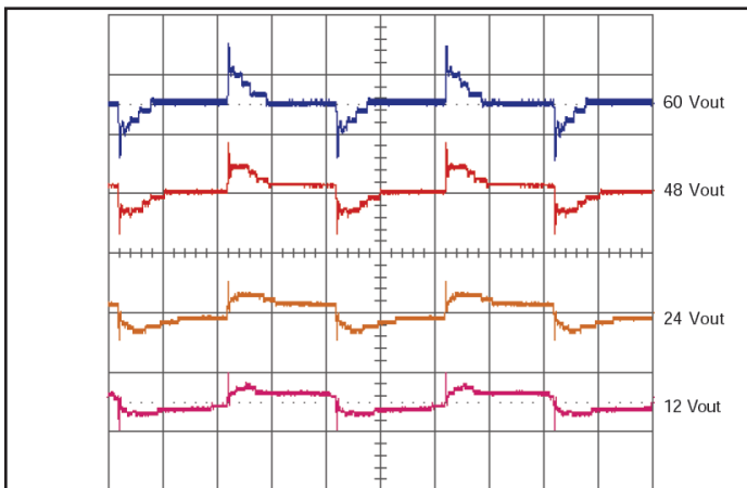
Figure 11: Output voltage response for 36V input; 12V, 24V, 48V, 60V output to step-change in load current (50-75-50% of Iout max; di/dt = 0.1A/μs). Load cap: 100μF, 100mΩ ESR tant, Ch 1-4: Vout (2V/div). Timescale: 5 ms/div.
