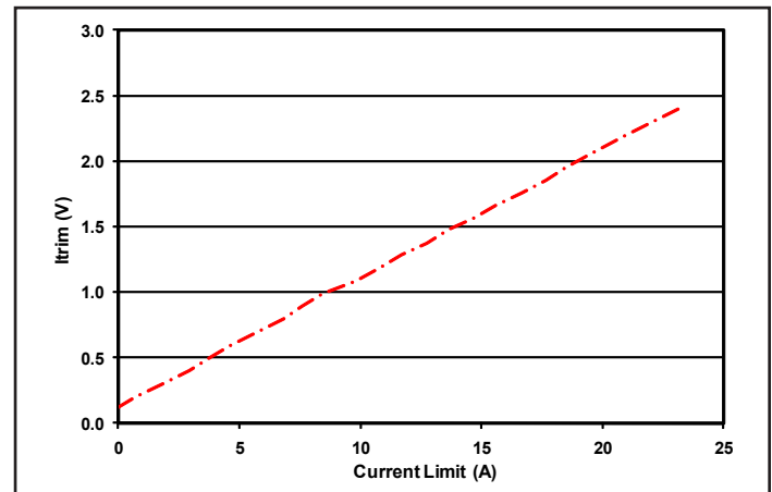
Figure 10: Current limit vs. Itrim pin voltage at 24V input and 13.8V output. Load capacitance: 100μF electrolytic cap. C option only.
